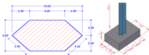
Figure-2. Models hexagonal pillar.
