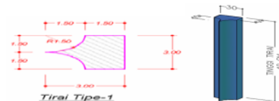
Figure-3. Shape Curtain Rectangler with Wedge Shape Curve (Rwwsc).
